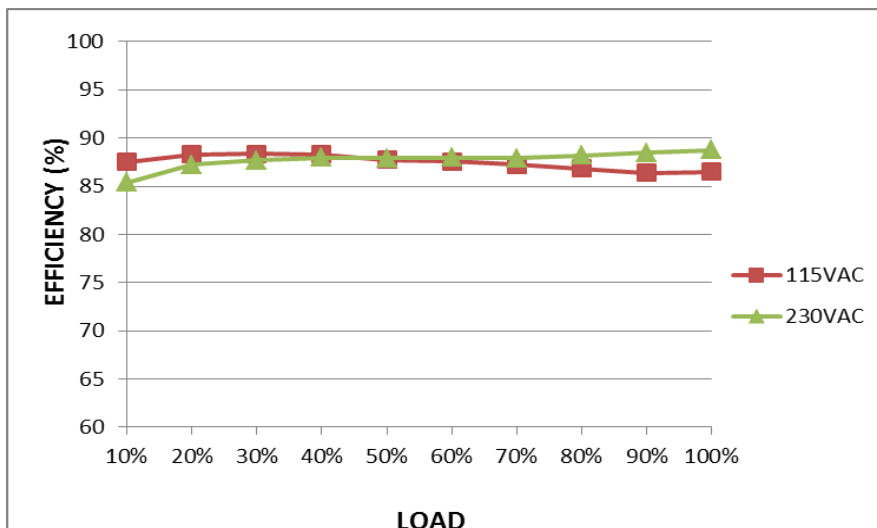
EFFICIENCY vs LOAD
