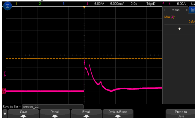
INPUT=48VDC @ FULL LOAD
